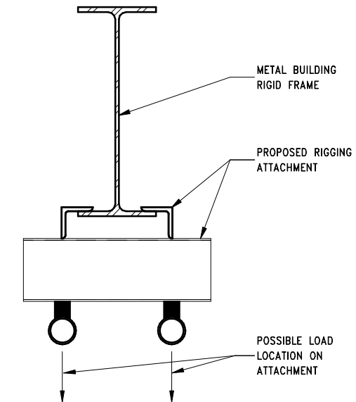
2 EXAMPLE RIGGING DETAIL S7-2 SCALE: 3/4" = 1'-0"
