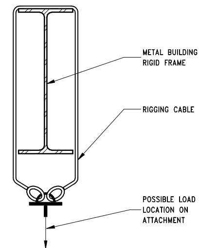
3 EXAMPLE RIGGING DETAIL S7-2 SCALE: 3/4" = 1'-0"
